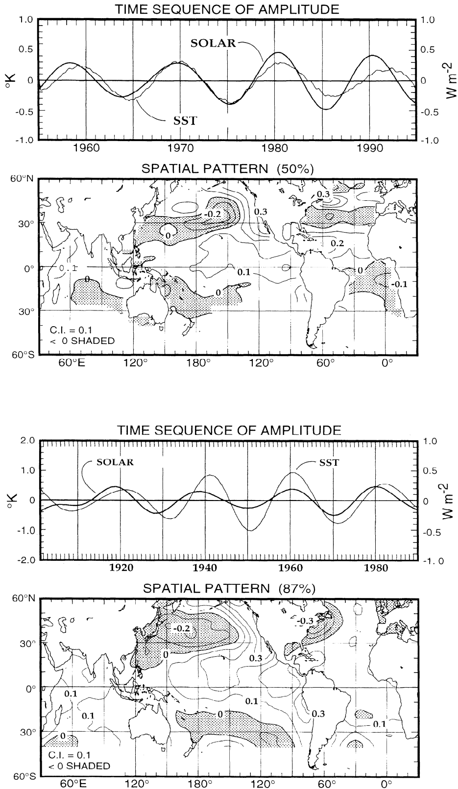
Figure 6. (top) Time sequence and spatial pattern of the first-mode empirical orthogonal function [Preisendorfer, 1988] applied to decadal BT sea surface temperature anomalies. This mode, together with its quadrature pair, explains 50% of decadal variance from 1955 to 1994. (bottom) Same as above, but for interdecadal GISST sea surface temperature anomalies, explaining 87% of interdecadal variance from 1901 to 1990. Superimposed on both time sequences are corresponding decadal and interdecadal anomalies of reconstructed solar irradiance anomalies at the top of the atmosphere. In each spatial pattern, negative weightings are shaded, and positive weightings are unshaded.
