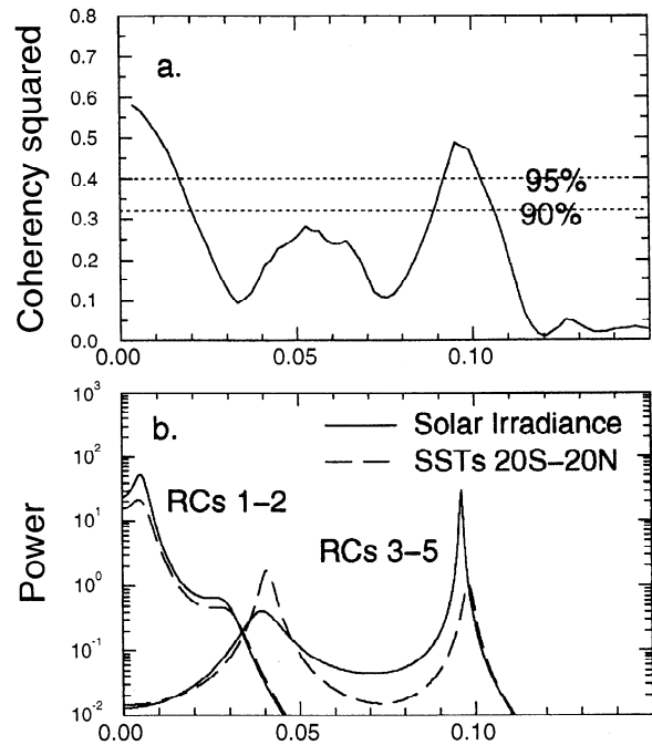
Figure 2. (a) Coherency spectrum for annual time sequences of global, 20°S–20°N, sea surface temperature and solar irradiance anomalies, 1900–1991. (b) Maximum entropy spectrum of leading reconstructed components (RCs) from two-channel singular-spectrum analysis (SSA) of sea surface temperature and solar-irradiance anomalies, with a window width of 27 years. Solar-irradiance fluctuations are at the top of the atmosphere in this and the next figure.
