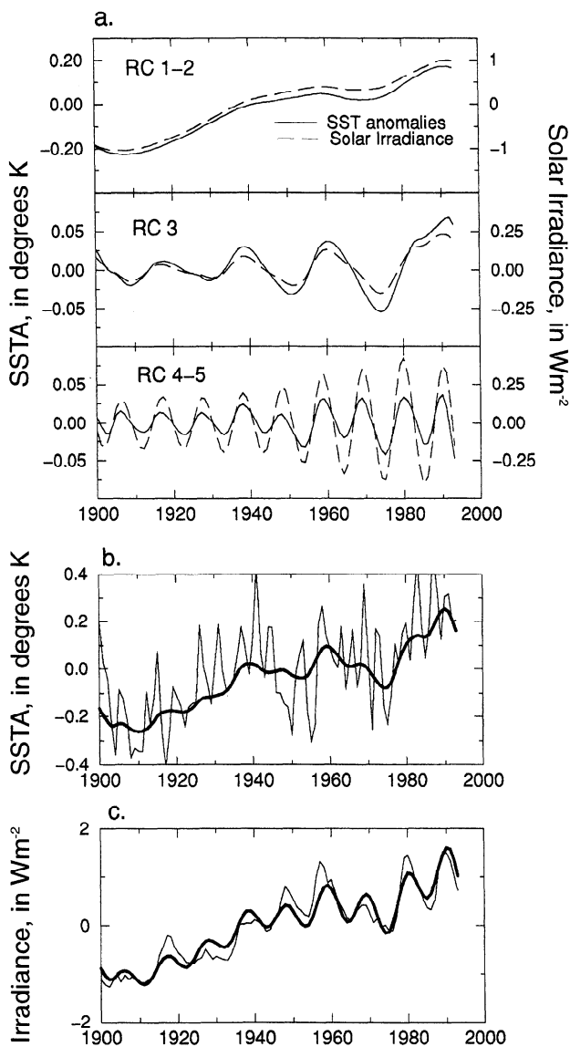
Figure 3. Reconstructed components (RCs) from two-channel SSA of annual global, 20°S–20°N, sea surface temperature and solar-irradiance anomalies, using a window width of 27 years: (a) RCs 1–2, RC 3, and RCs 4–5; (b) RCs 1–6 of sea surface temperature anomalies (heavy curve) and unfiltered anomalies (light curve); and (c) RCs 1–6 of solar irradiance anomalies (heavy curve) with unfiltered anomalies (light curve).
