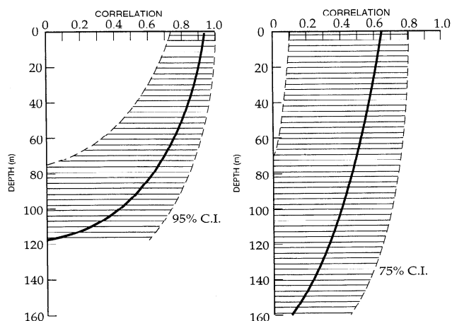
Figure 5. (left) Correlation as a function of depth between global-average BT upper ocean temperature and reconstructed solar irradiance anomalies for 1955–1994 on decadal scales. (right) Correlation as a function of depth between global-average BT upper ocean temperature and solar irradiance anomalies for 1955–1994 on interdecadal scales. Confidence intervals are lined, computed on the basis of Fischer's Z transform [Snedecor and Cochran, 1980].
