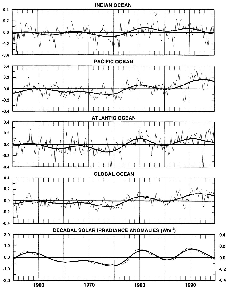
Figure 4a. Time sequences of decadal sea surface temperature anomalies (in kelvins) averaged over Indian, Pacific, Atlantic, and global oceans from the BT data base from 1955 to 1994. Light curves give individual monthly mean anomalies, and heavy curves give low-pass-filtered versions (i.e., with half-power points at 7 years). Also displayed are time sequences of reconstructed solar irradiance and its corresponding low-pass-filtered version for the same period. In the bottom panel, two values of solar irradiance are given; on the left are values at the top of the atmospheres ( S_T ); on the right are global-average estimates at the sea surface, the solar insolation (i.e., S = 0.7(S_T/4) ). To avoid loss of at the ends of each time sequence due to low-pass filtering, maximum-entropy spectral analysis was applied [Andersen, 1974] using spectral coefficients to extend both ends of each sequence by half the filter width.
