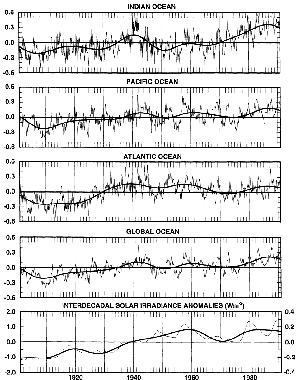
Figure 4b. Same as Figure 4a, but for the interdecadal GISST data set from 1900 to 1991, and with low-pass-filtered versions computed with half-power points at 15 years.
