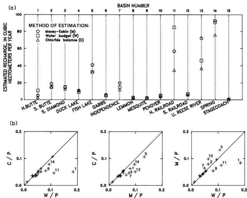
Fig. 4. Comparisons of estimates of natural recharge for fifteen basins in Nevada, using the Maxey-Eakin, water budget, and chloride-balance methods. (a) Rates of natural recharge; (b) ratios of estimates to precipitation rate ( P ) in recharge-source areas. Ratios indicated in terms of single-letter estimate designations in explanation, Fig. 4a, and outlying points are labeled with the same basin numbers as at top of Fig. 4a and Table 2.
